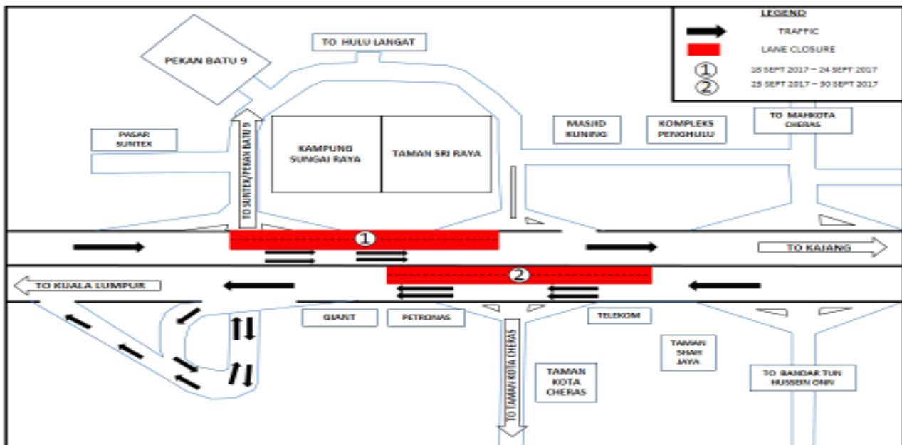
MAP 2: LANE CLOSURE AT KM 13.3 UNTIL KM 14.7 CHERAS-KAJANG HIGHWAY (KAJANG AND KUALA LUMPUR-BOUND)
