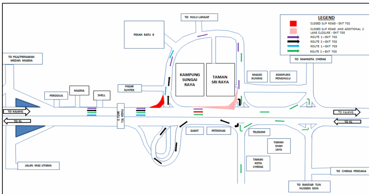
MAP 5: SLIP ROAD CLOSURE AT EXIT 702 AND EXIT 703, CHERAS-KAJANG HIGHWAY (KAJANG AND KUALA LUMPUR BOUND)
