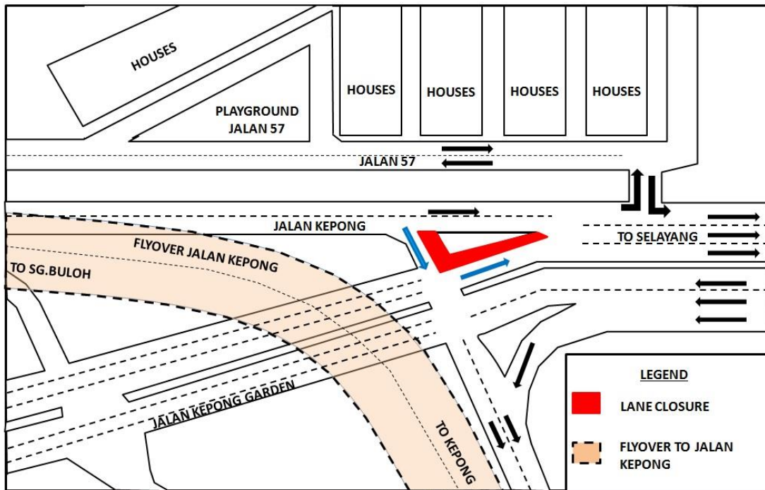
MAP 3 : LANE CLOSURES UNDERNEATH MRR2 FLYOVER (KEPONG-BOUND AND SELAYANG-BOUND)
