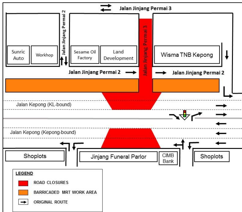
MAP 1 : NIGHT LANE CLOSURES BY STAGES ALONG JALAN JINJANG PERMAI 3 & JALAN KEPONG (KEPONG-BOUND AND KL-BOUND)
